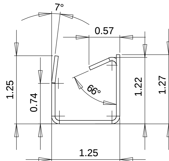
Profile [1:1]
